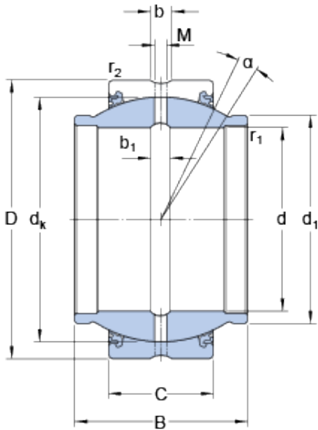
GEZM 600 ESX-2LS Bearing 2D drawings and 3D CAD models
